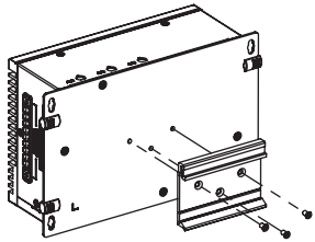
DIN-Rail Assembly
