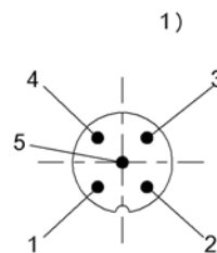
1) View towards connector 2) Male 5-pin/ Function
