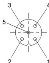
1) View towards connector 2) Female 5-pin/ Function
