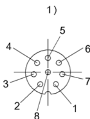
1) View towards connector 2) Socket 8-pin/ Function
